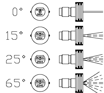
FIGURE A. ADJUSTABLE NOZZLE
