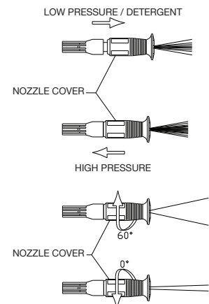
FIGURE A. ADJUSTABLE NOZZLE
